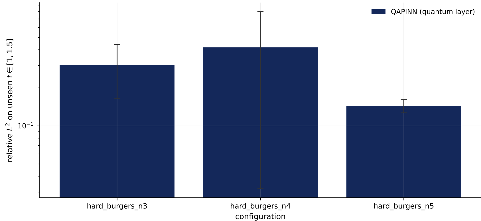
Generalization beyond training domain (mean \pm s.d., 3 seeds)
